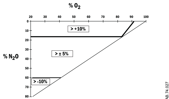
Figure 11-7 • Gas composition related errors
