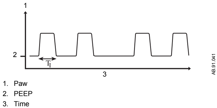
Figure 11-4 • PSVPro diagram
