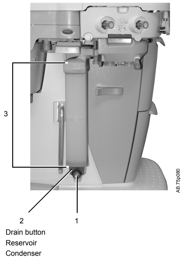
Figure 3-5 • Condenser
